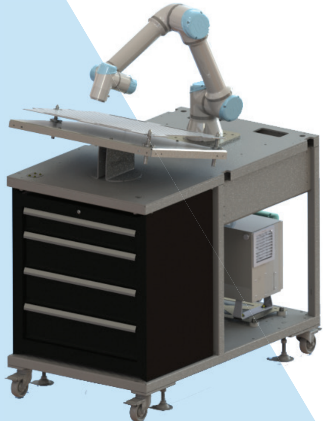
Mobile Cart
