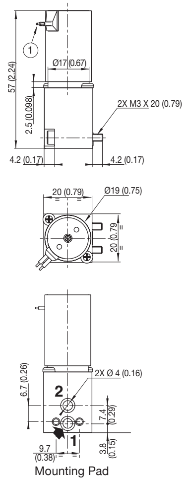
LS202A516 (POM)
