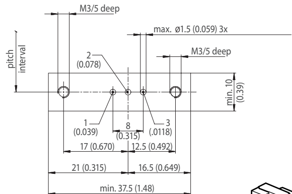
Mounting Pad
