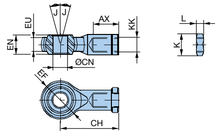
Dimensions — mm
