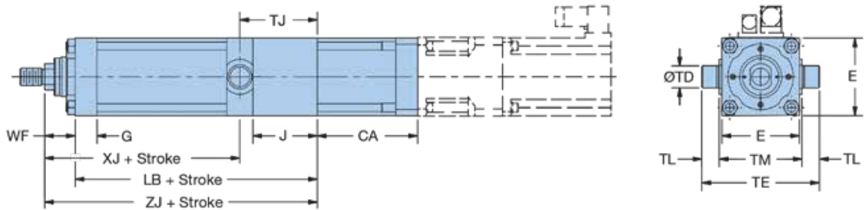
Dimensions — mm (in)
