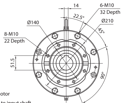
Hollow Mount
