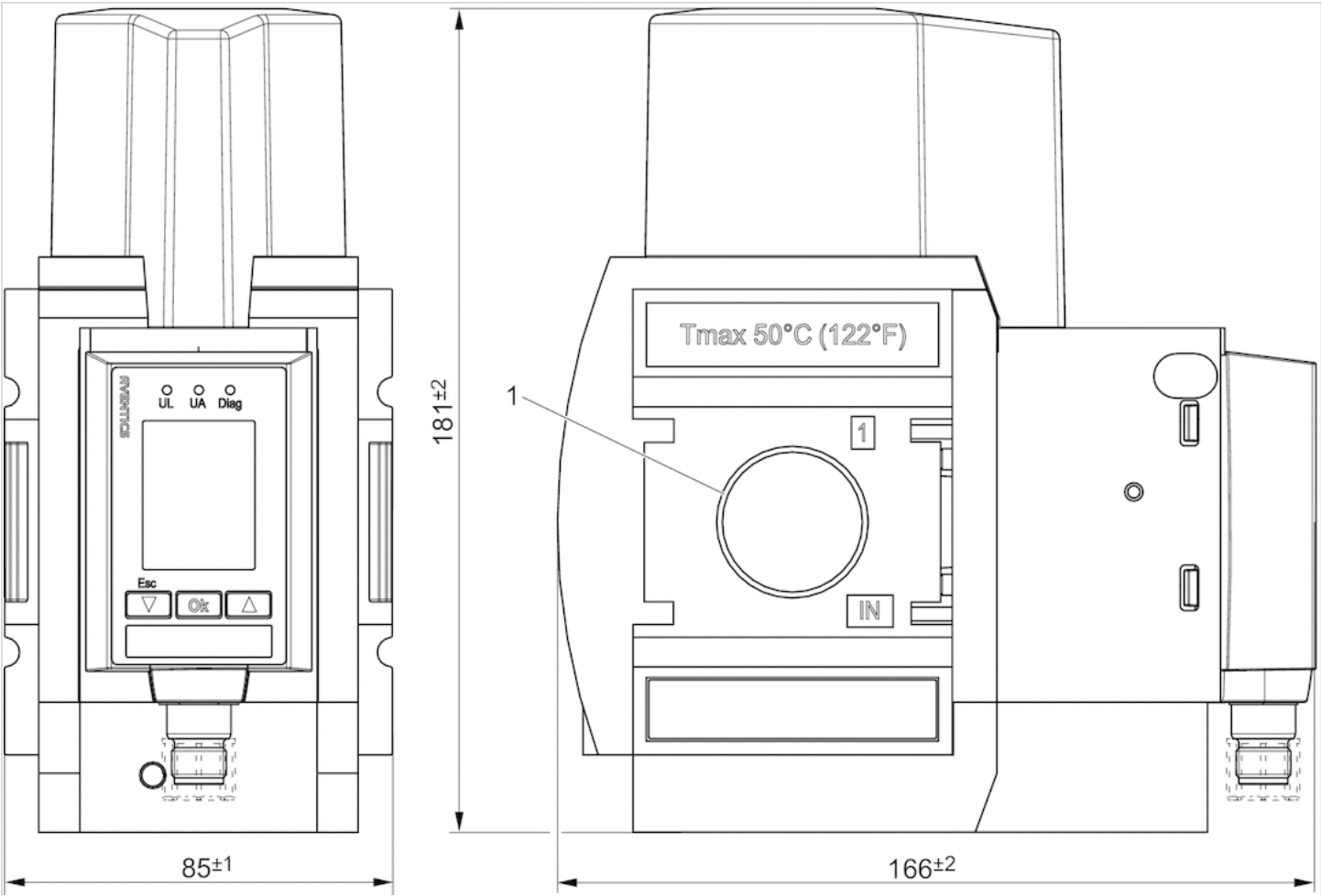
1) Connection thread
