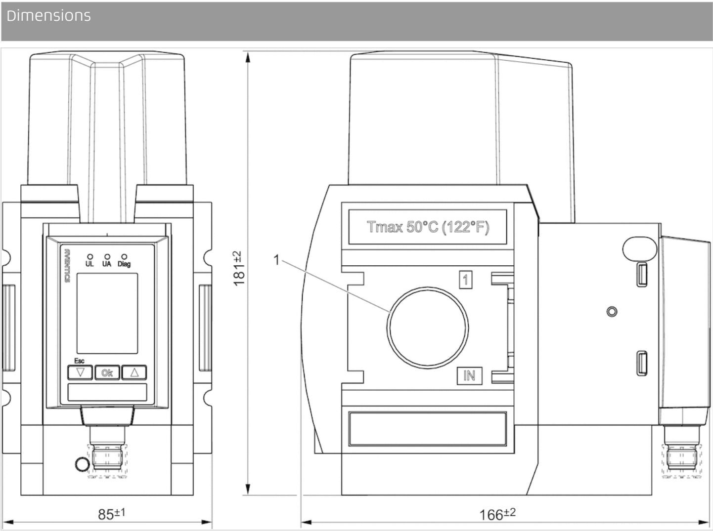
1) Connection thread
